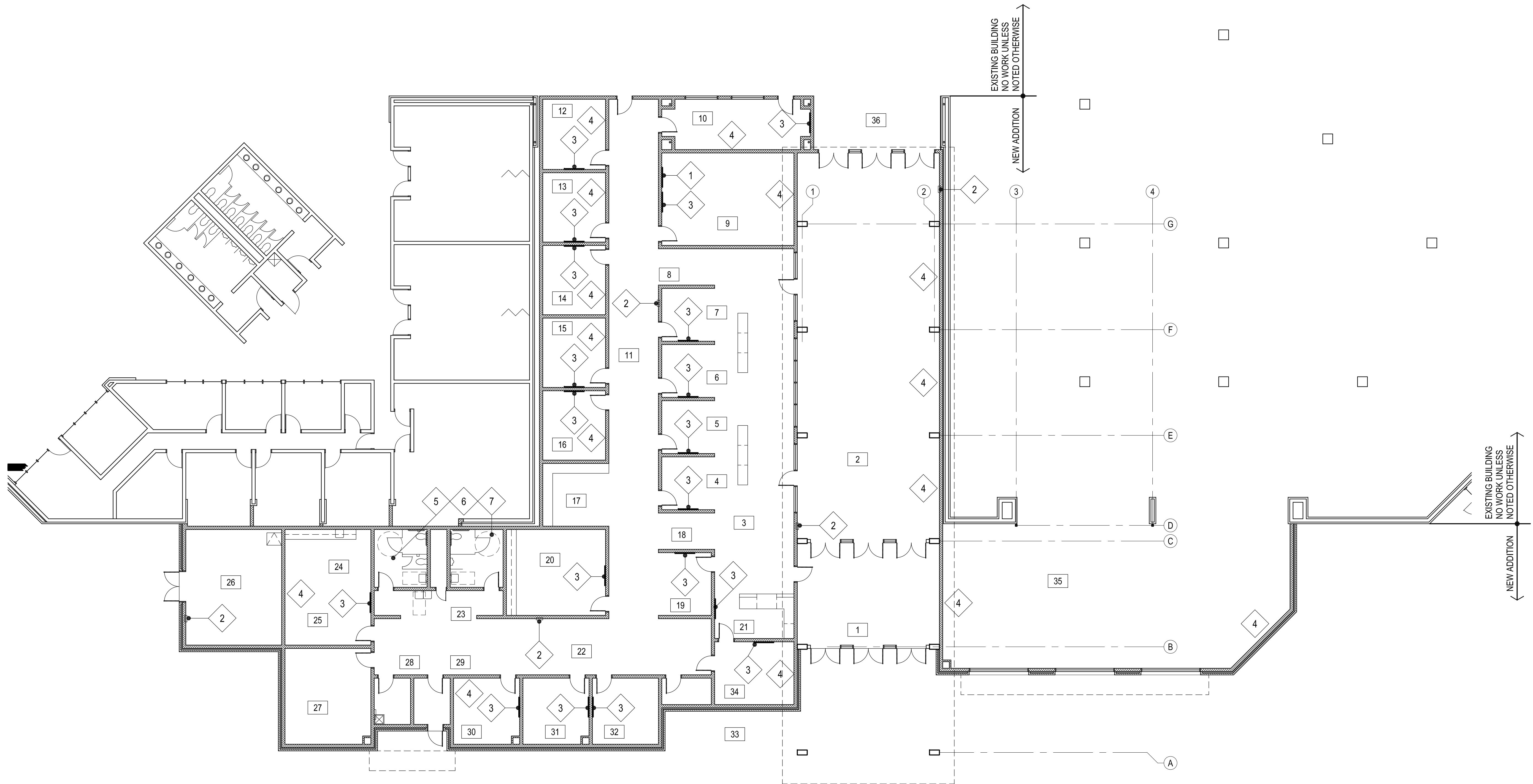
EQUIPMENT FLOOR PLAN 3/32" = 1'-0"
