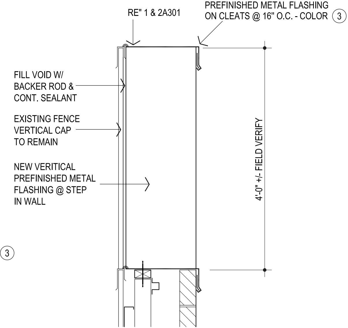
VERTICAL FLASHING @ STEP IN FENCE 1" = 1'-0"
