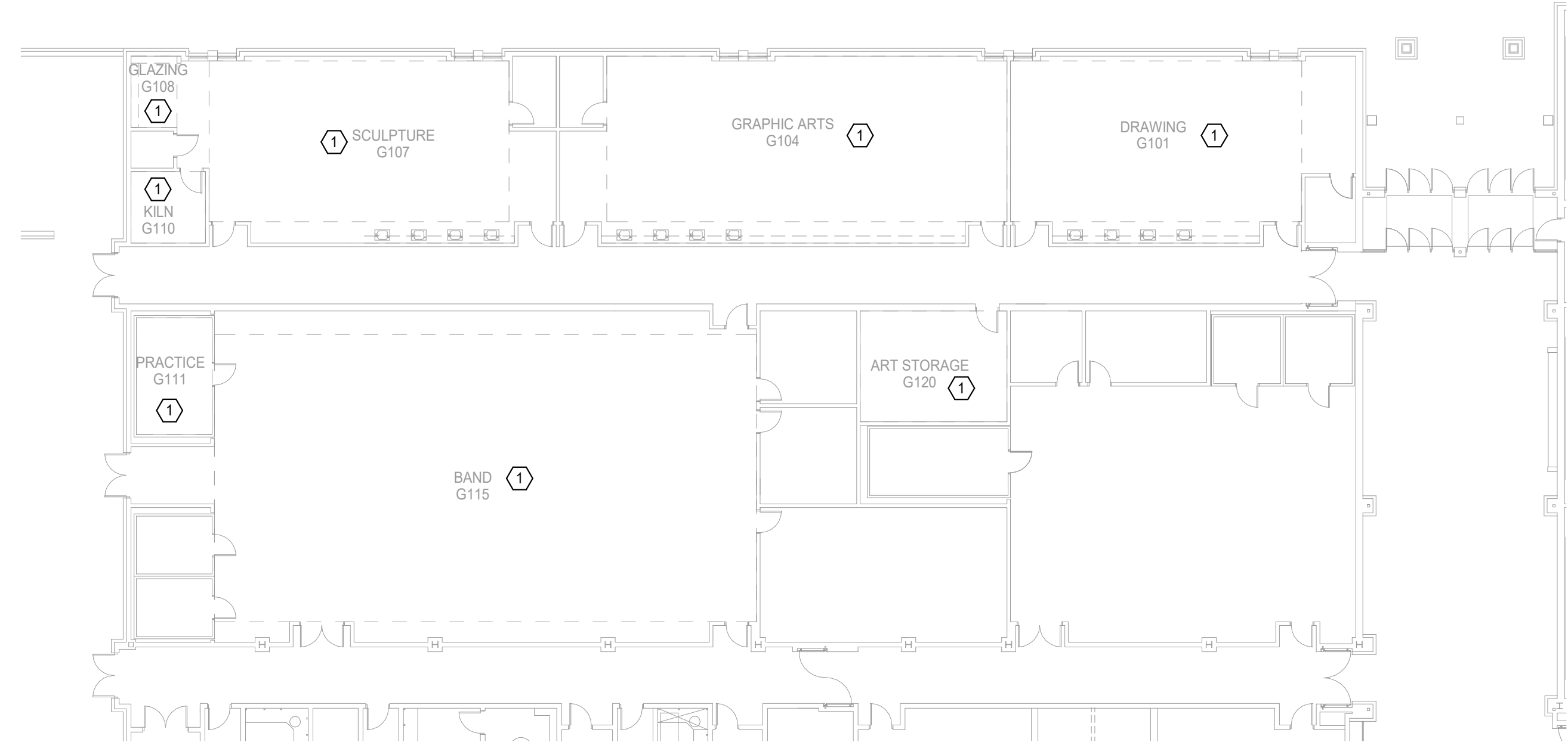
1 MECHANICAL FLOOR PLAN - LEVEL 1 AREA G Scale: 1/16" = 1'-0"
