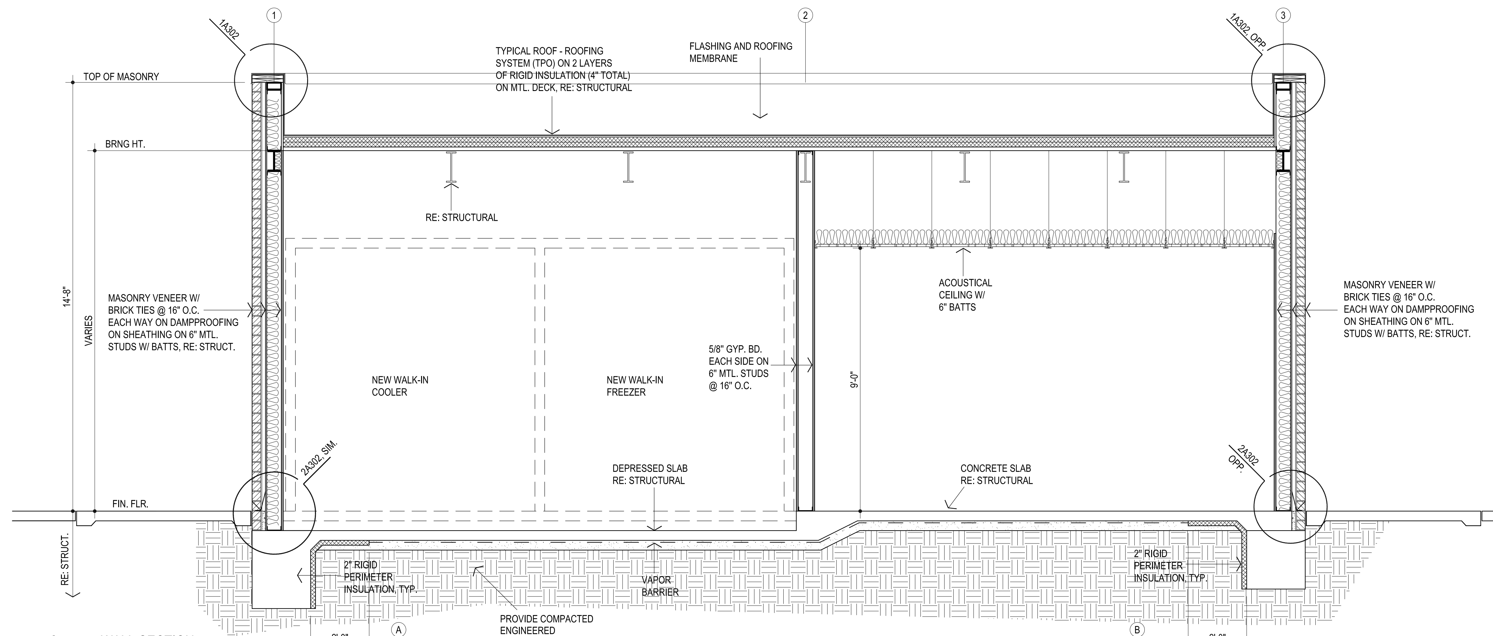
1 WALL SECTION 1/2" = 1'-0"
