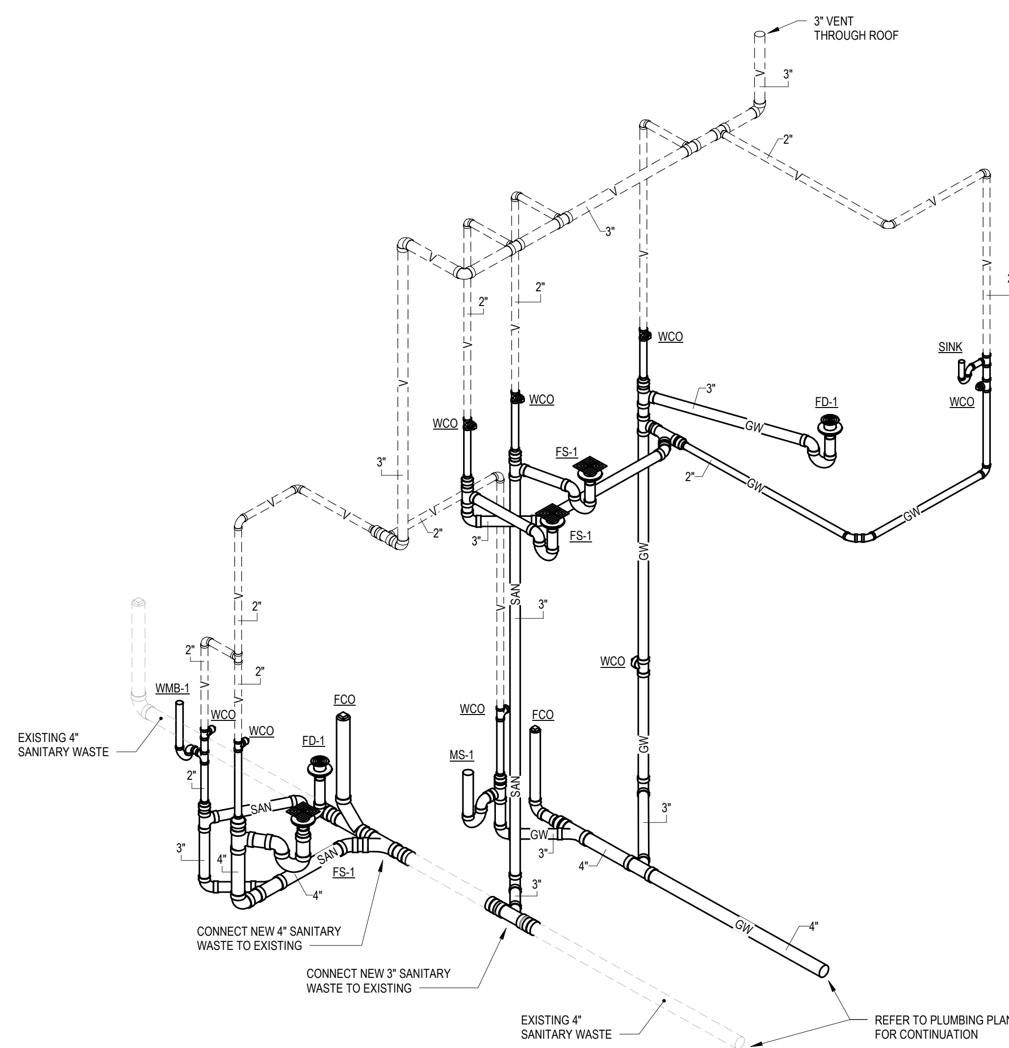
2 WASTE AND VENT RISER - MEZZANINE AND BACK OF HOUSE
