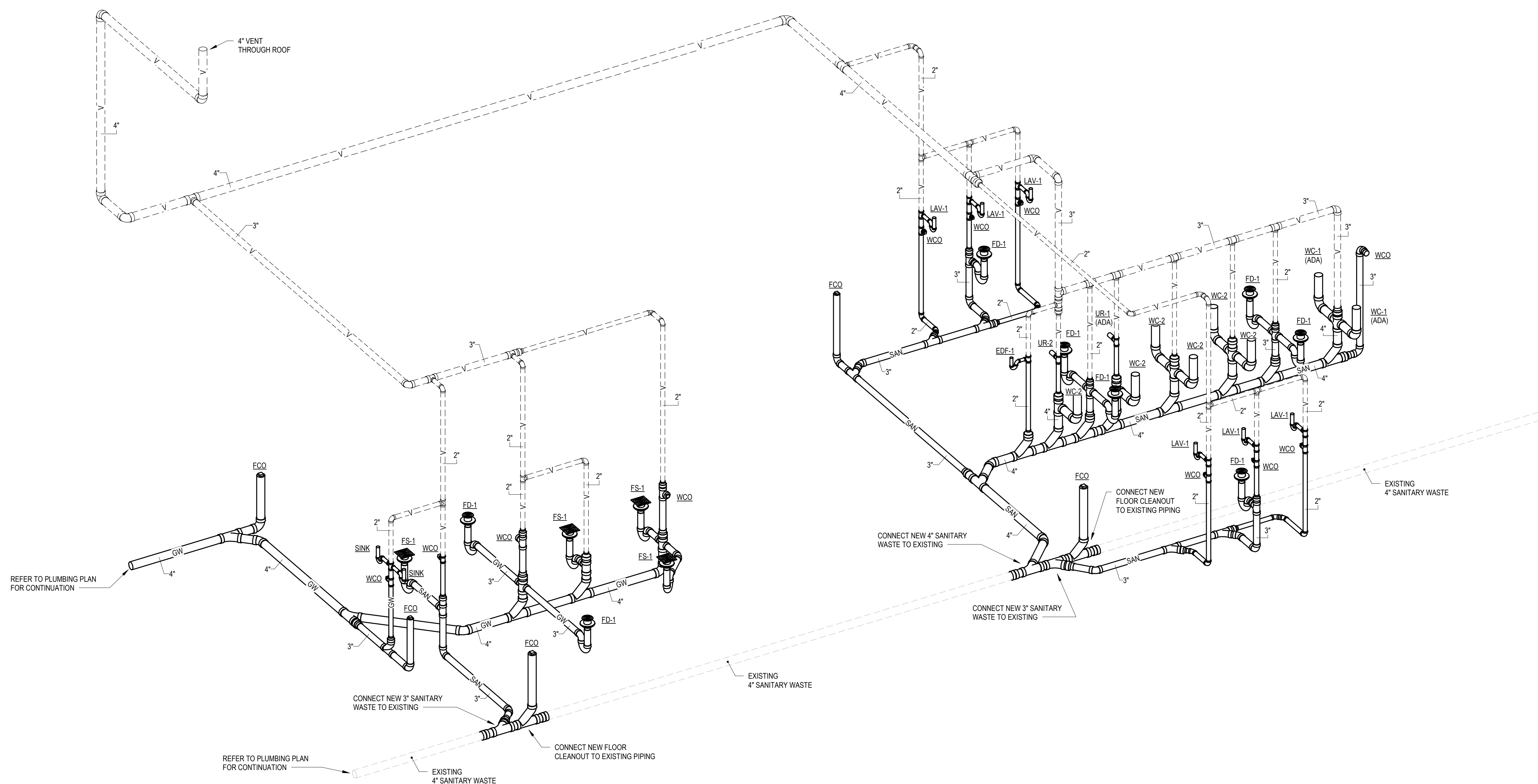
1 WASTE AND VENT RISER - RESTROOMS AND CAFE
