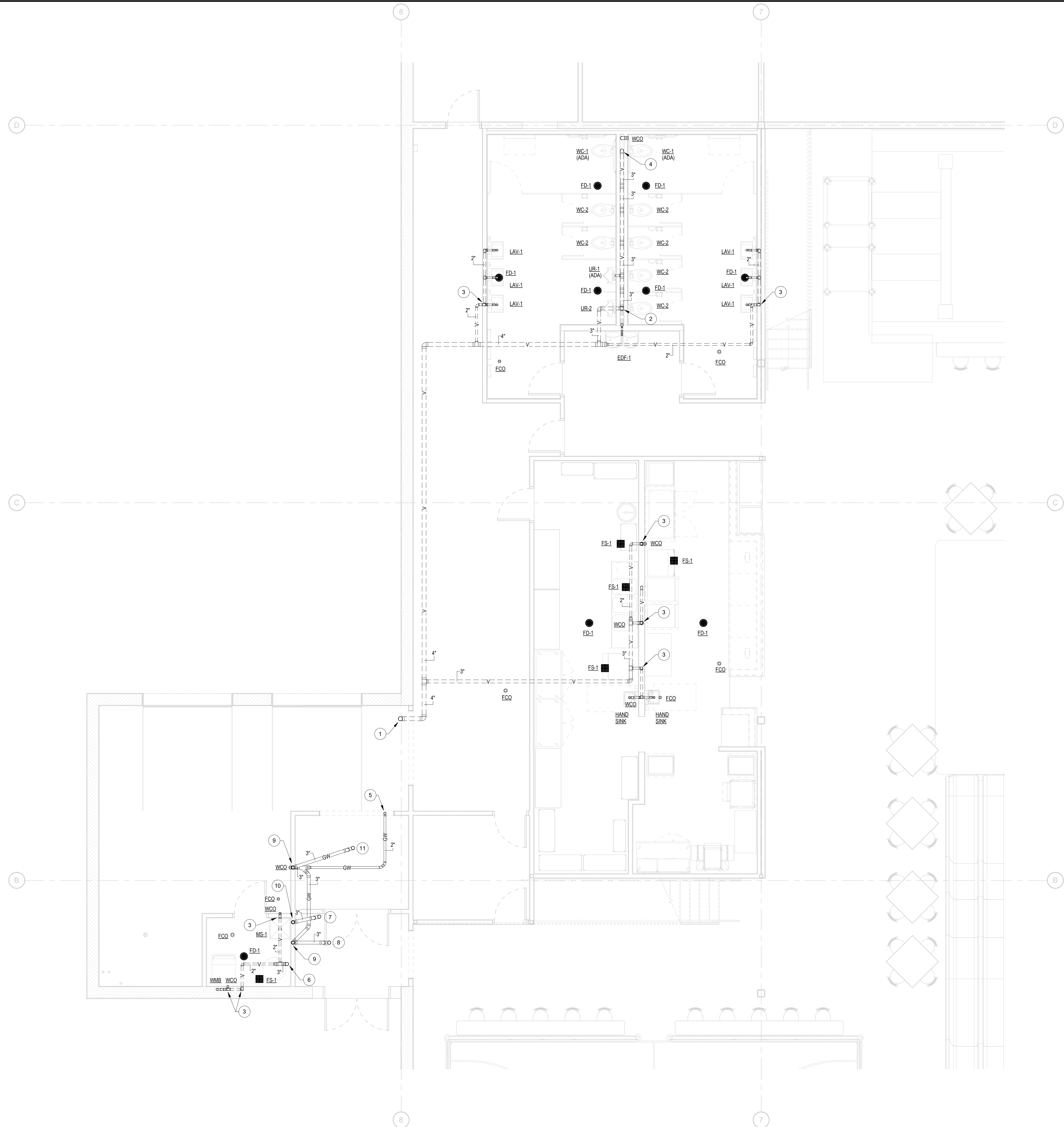
1 PLUMBING FLOOR PLAN - AREA A P101A 1/4" = 1'-0"
