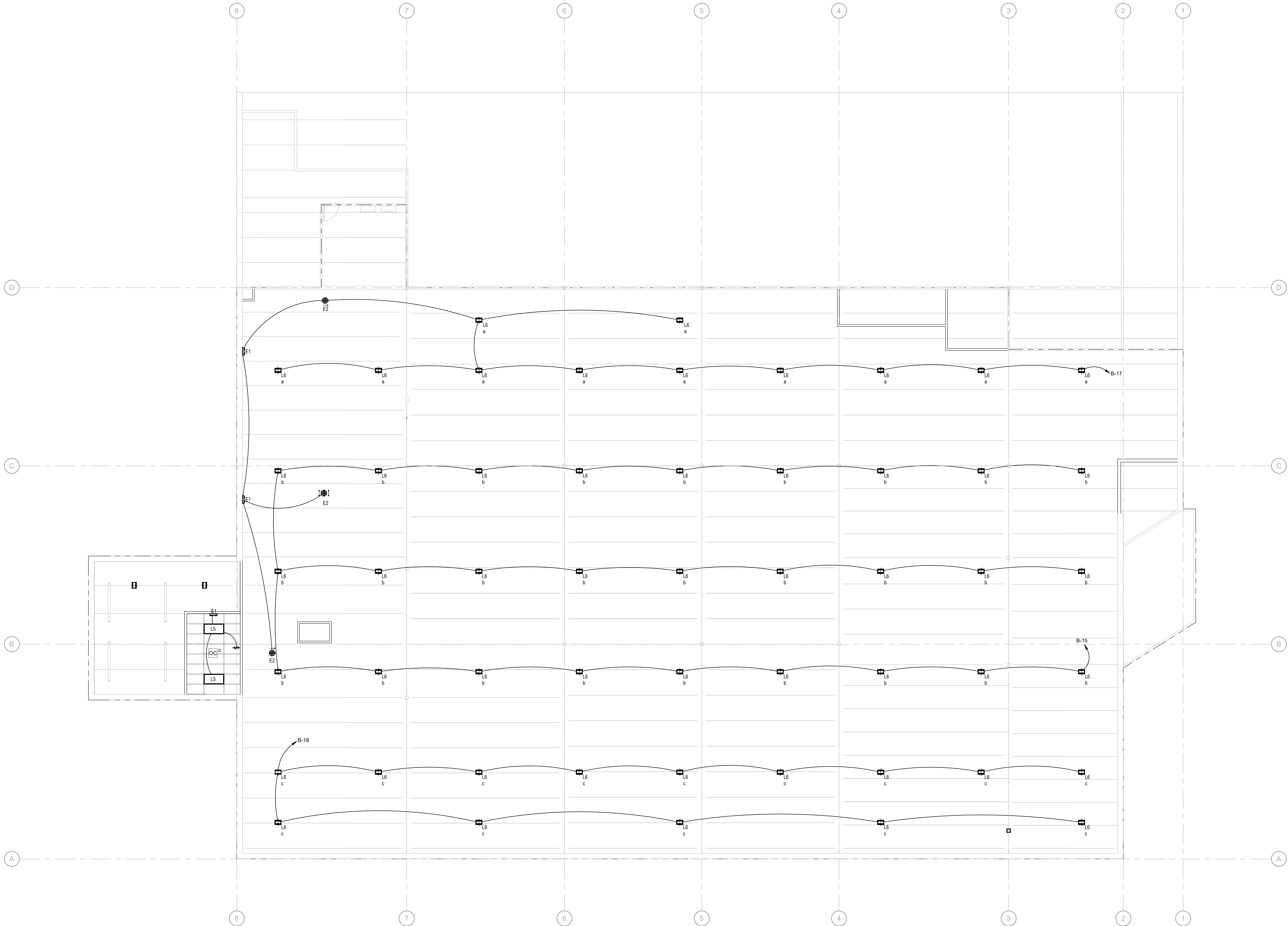
1 ELECTRICAL MEZZANNINE LIGHTING PLAN E201 1/8" = 1'-0"
