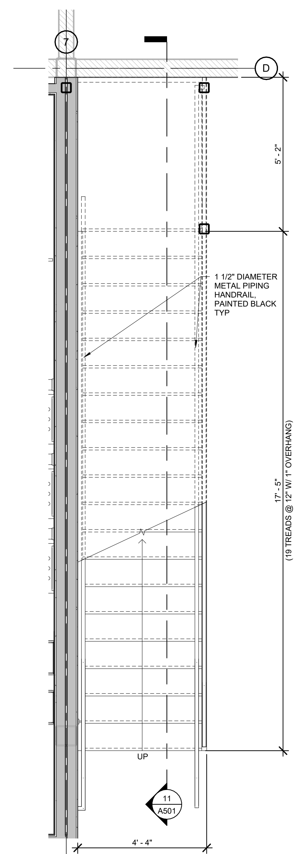
1 ENLARGED STAIR PLAN SCALE: 1/2" = 1'-0"
