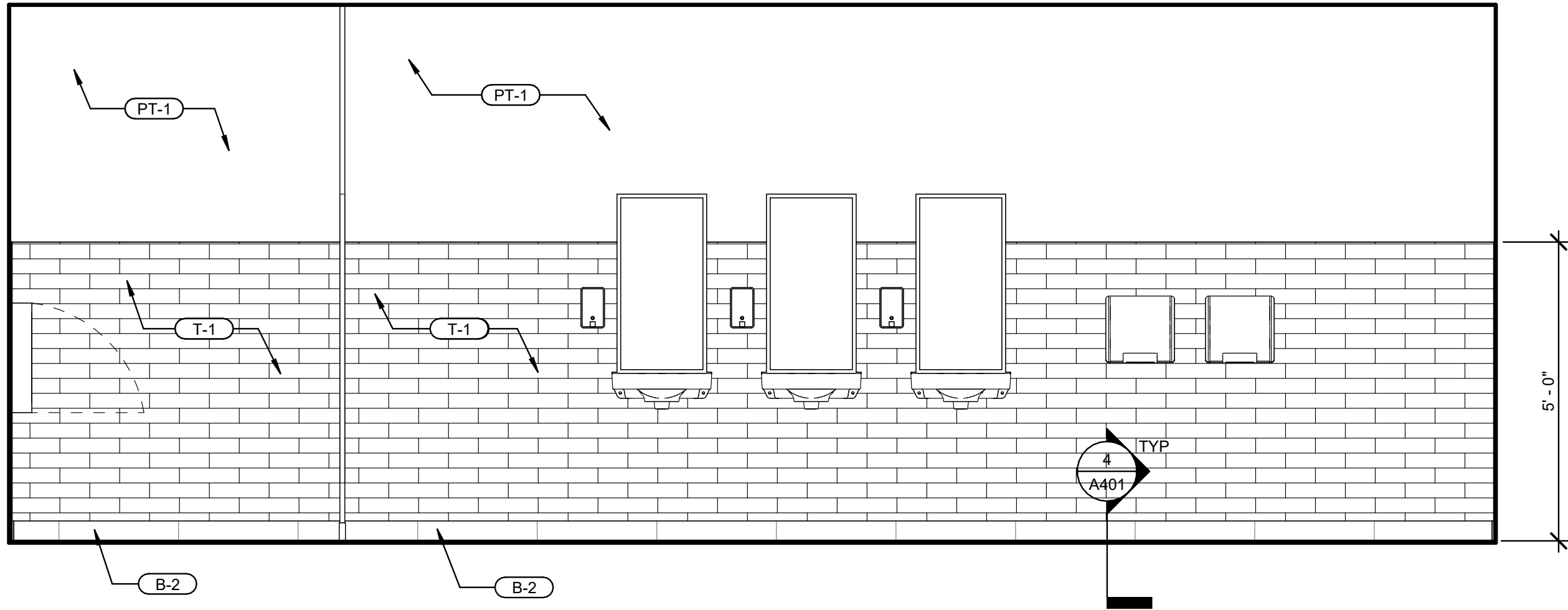
③ WOMEN SCALE: 1/2" = 1'-0"
