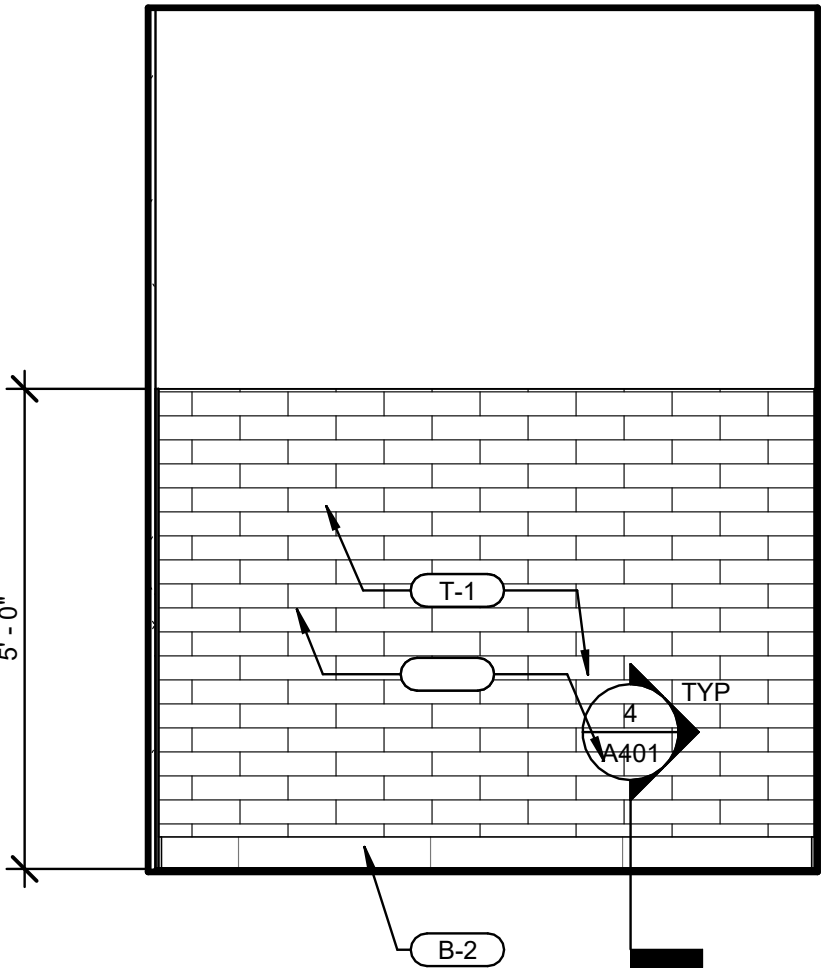
④ WOMEN SCALE: 1/2" = 1'-0"
