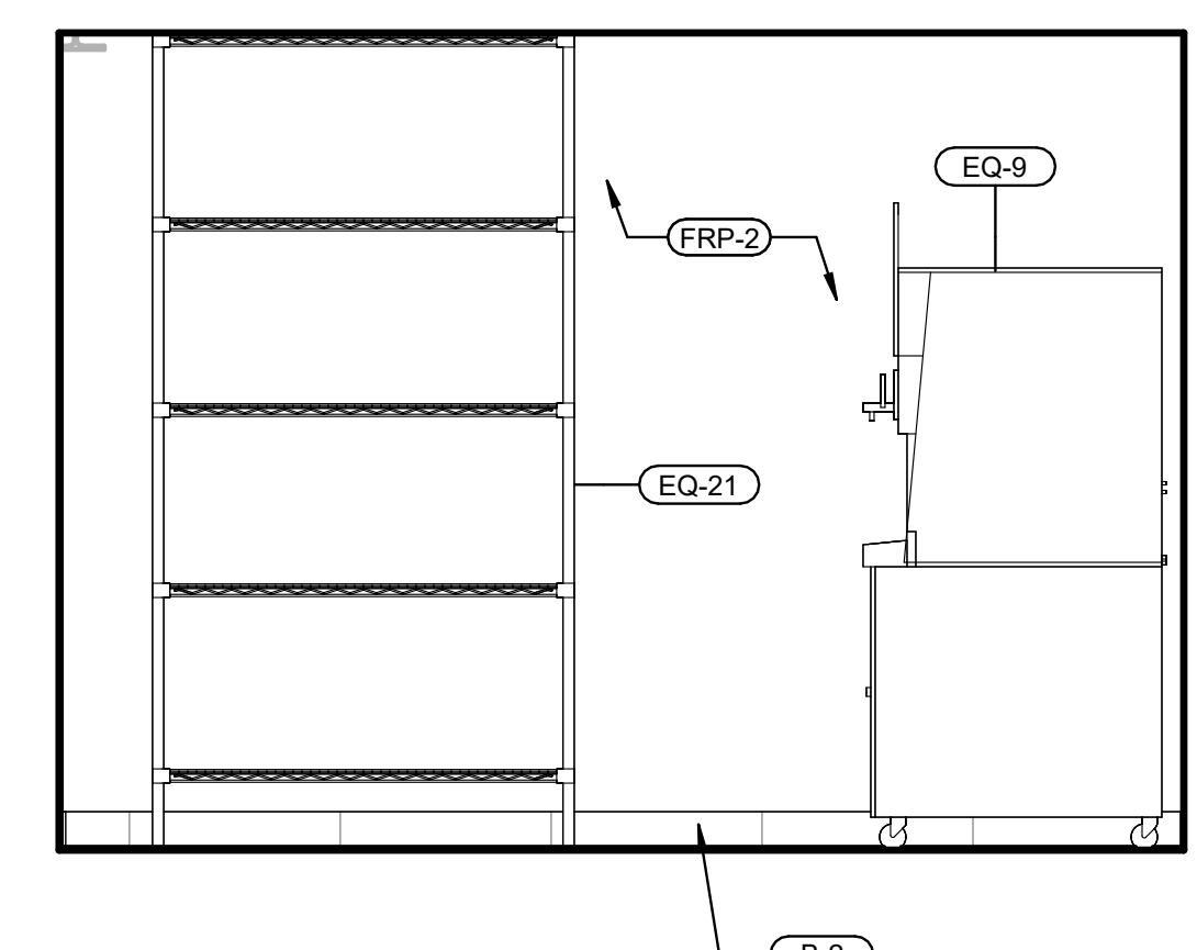
⑥ PARTY HOST SCALE: 1/2" = 1'-0"
