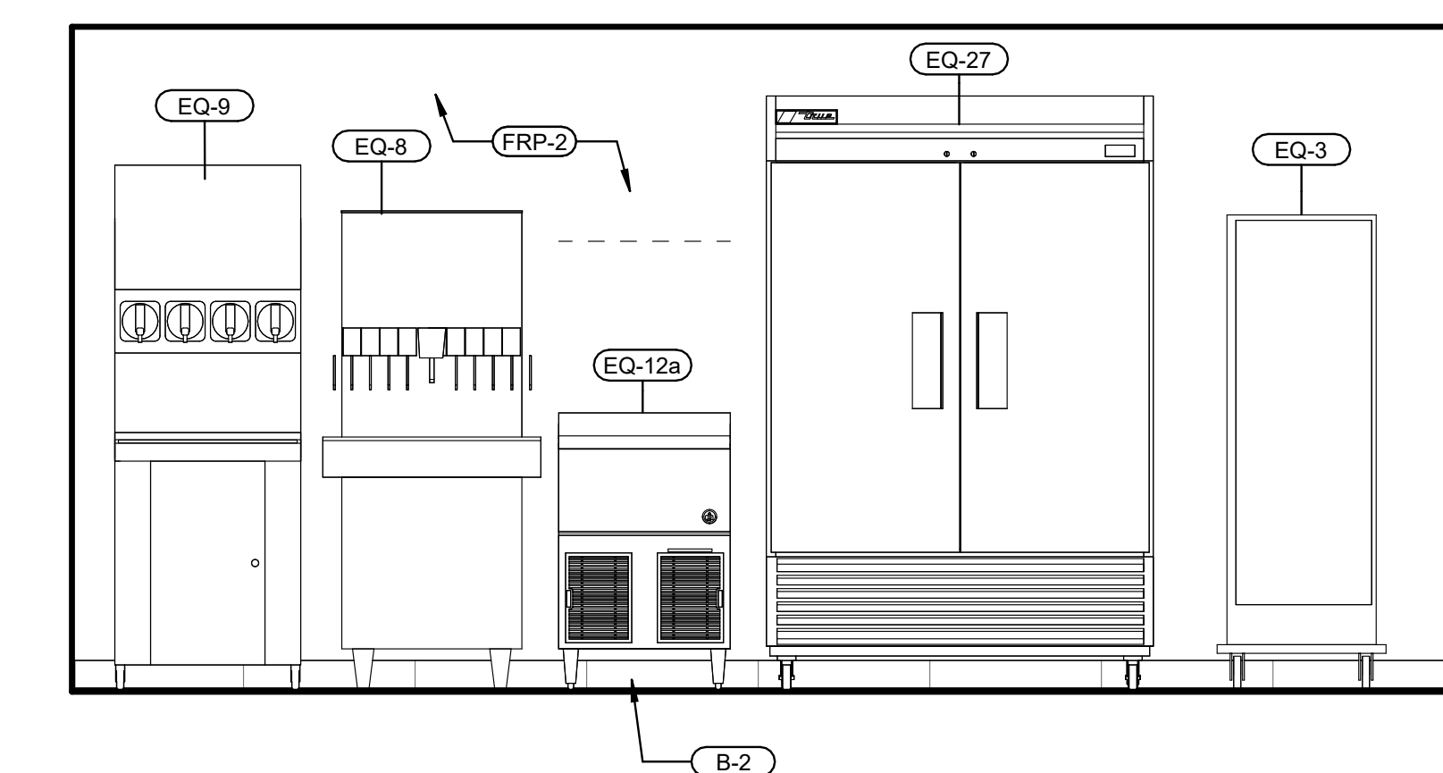
⑦ PARTY HOST SCALE: 1/2" = 1'-0"
