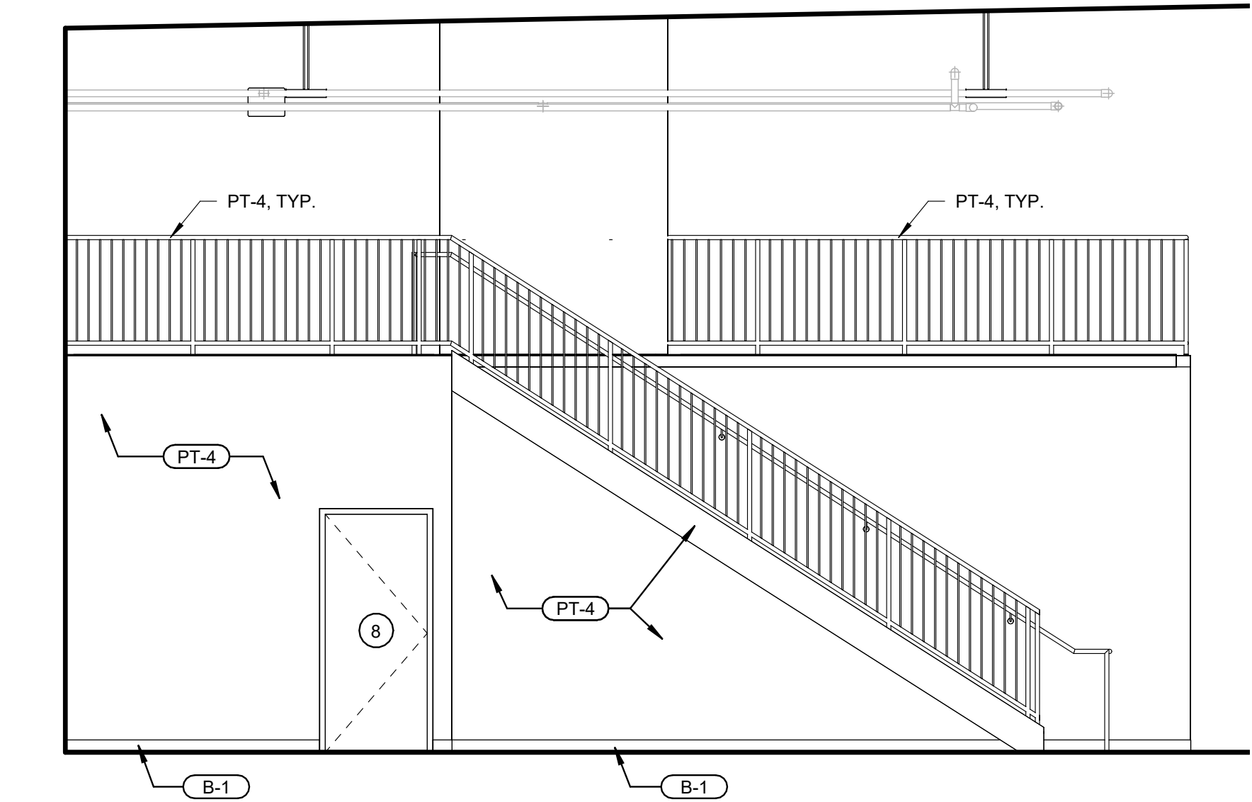
3 EXERCISE SCALE: 1/4" = 1'-0"
