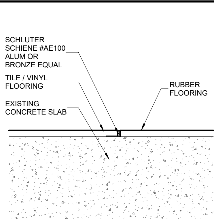
② TILE / VINYL FLOOR TO RUBBER FLOOR SCALE: 3" = 1'-0"
