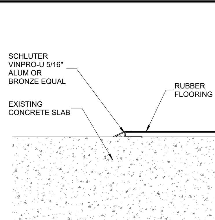
③ RUBBER FLOORING TO CONCRETE SCALE: 3" = 1'-0"
