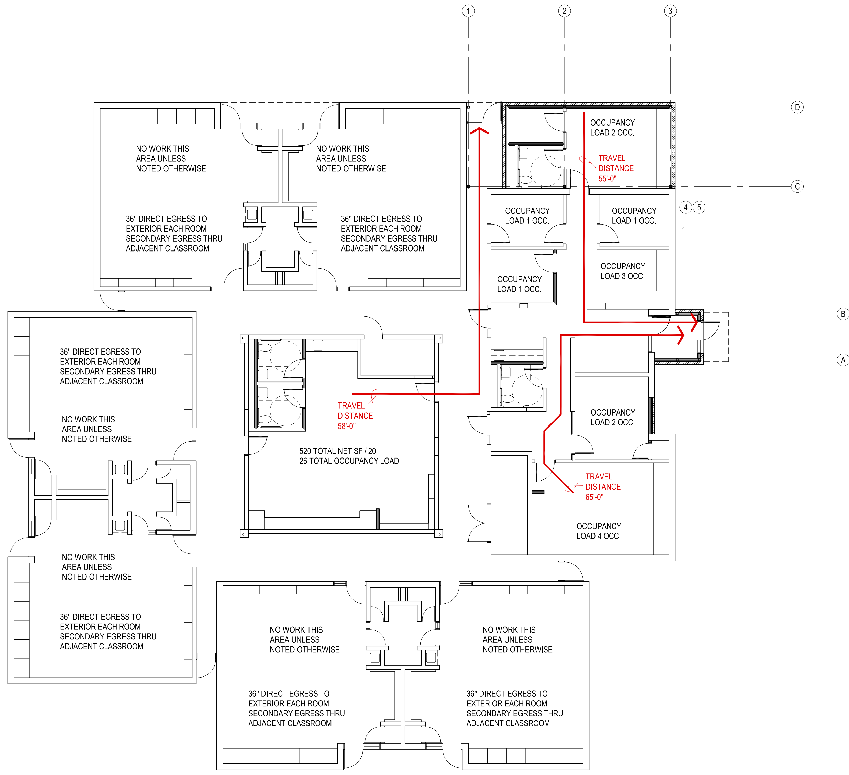
1 EGRESS PLAN 1/8" = 1'-0" NORTH
