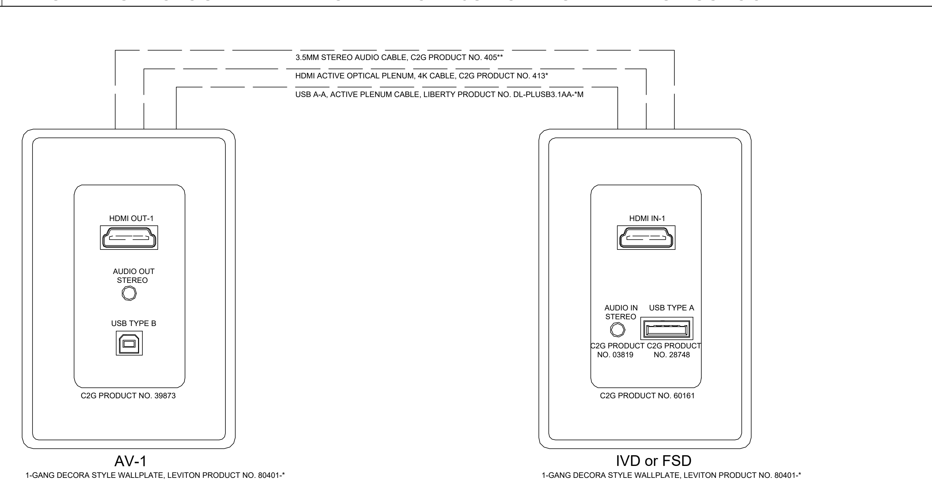
02 TYPICAL 'IVD' 'AV-1' OUTLET DETAIL
