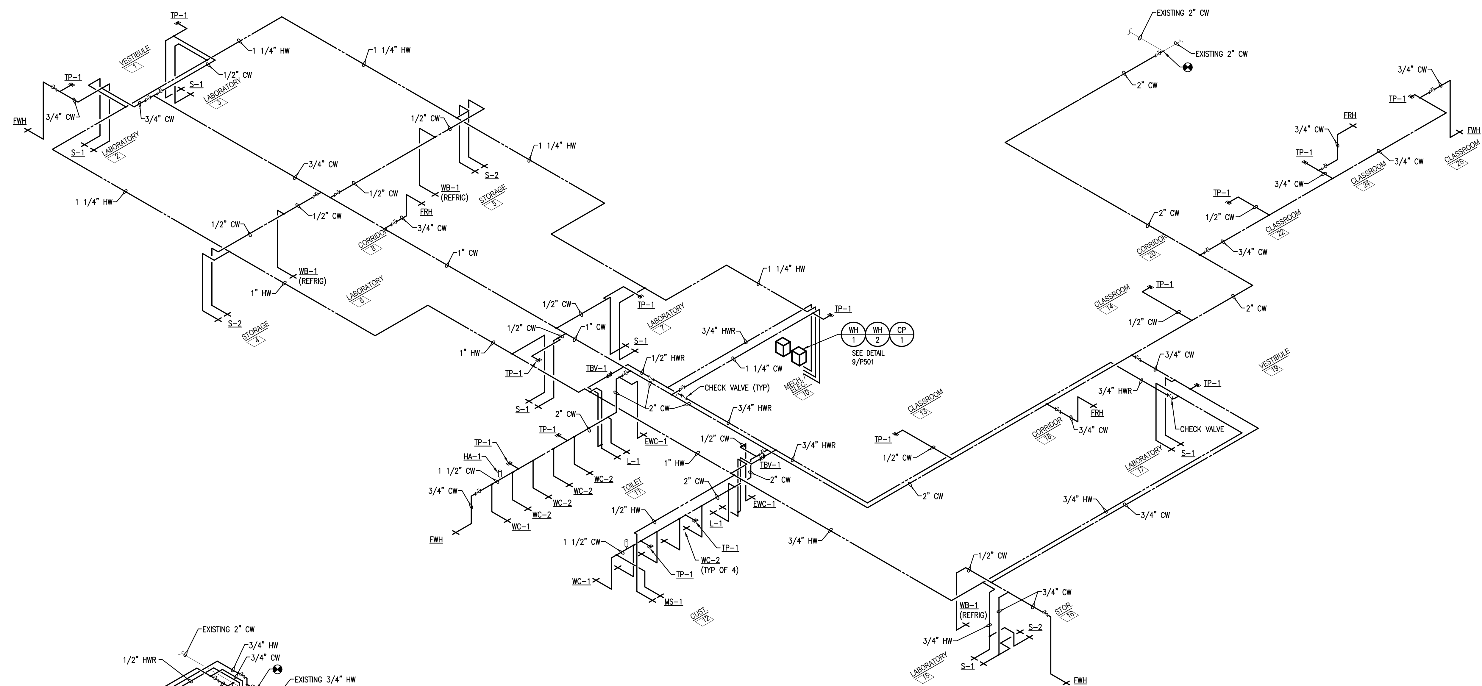
1 PLUMBING ISOMETRIC - WATER SUPPLY - AREAS A, B & C NO SCALE
