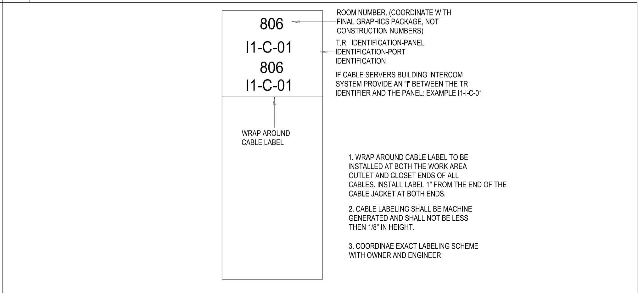
06 CABLE LABEL DETAIL NOT TO SCALE
