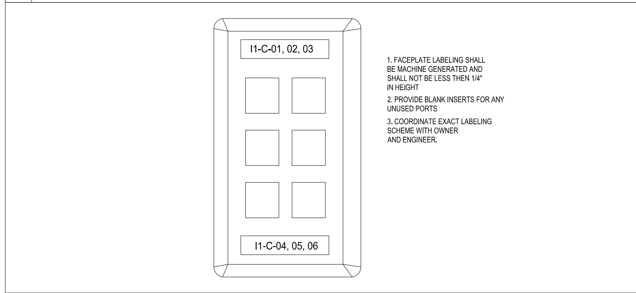
05 FACEPLATE LABEL DETAIL NOT TO SCALE
