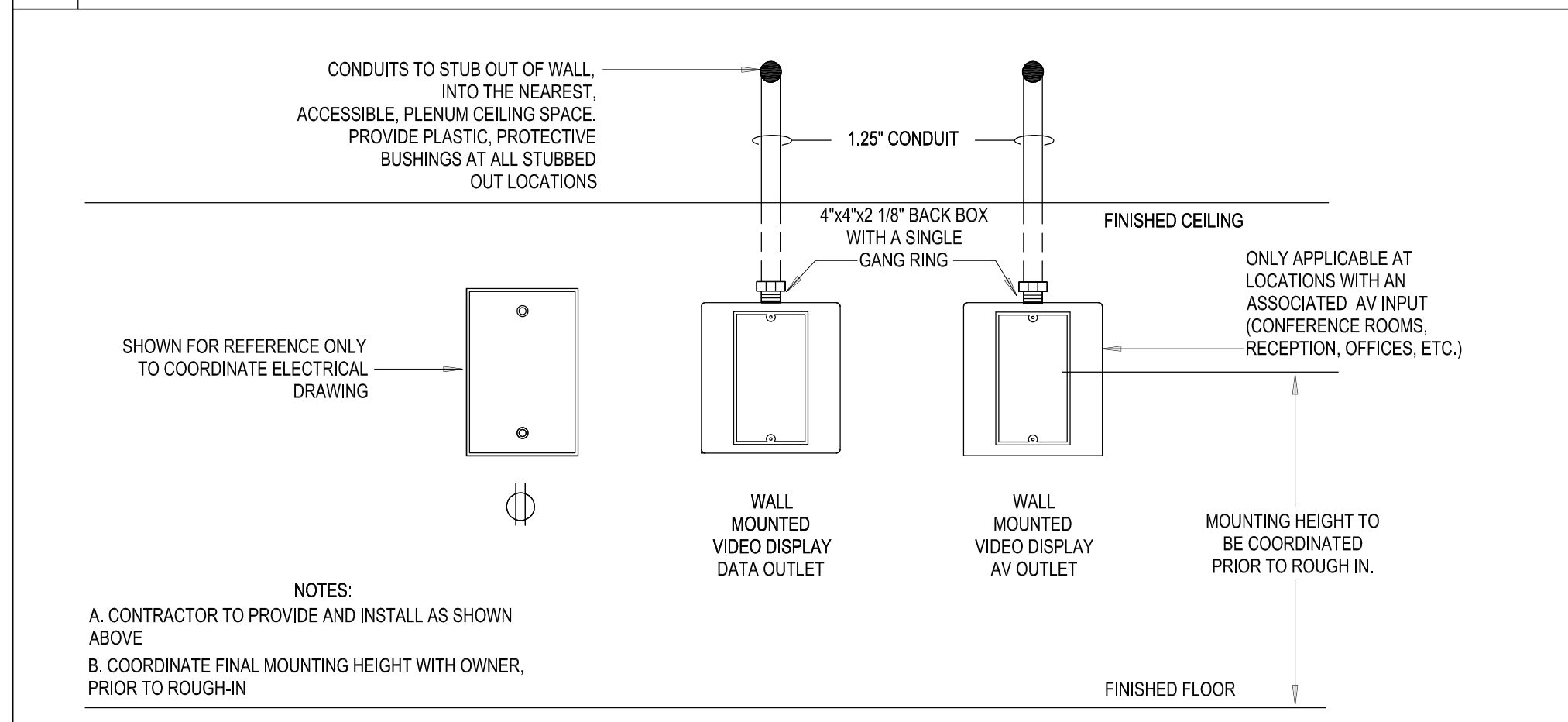
03 RACEWAY DETAIL - WALL MOUNTED DISPLAY NOT TO SCALE
