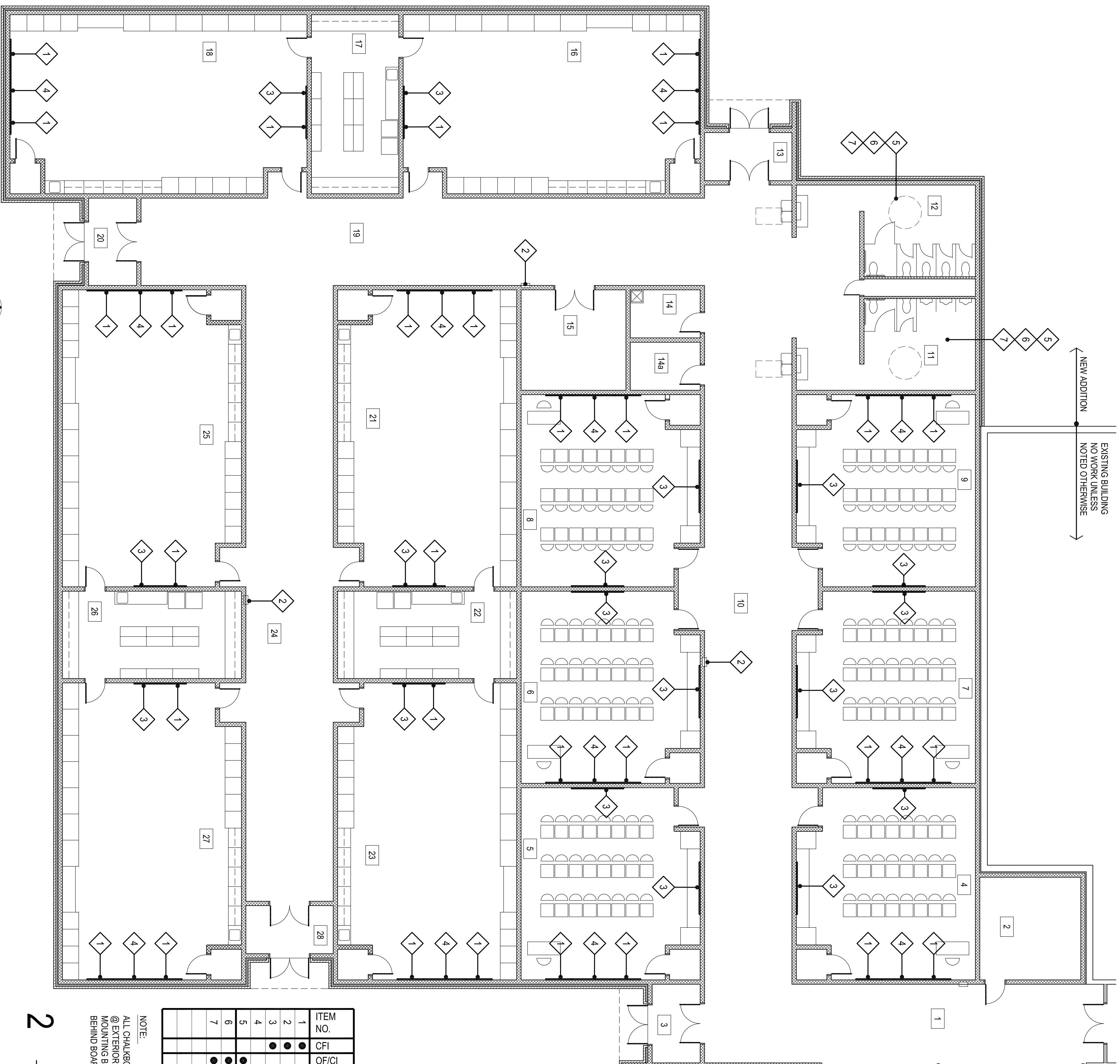
1 EQUIPMENT FLOOR PLAN 1/8" = 1'-0"
